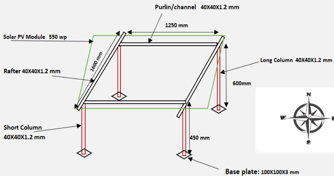
★ Top View of Portable Solar panel with Mounting Structure
